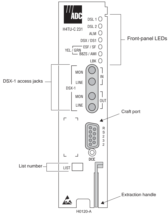
Figure 1. H4TU-C Front Panel
