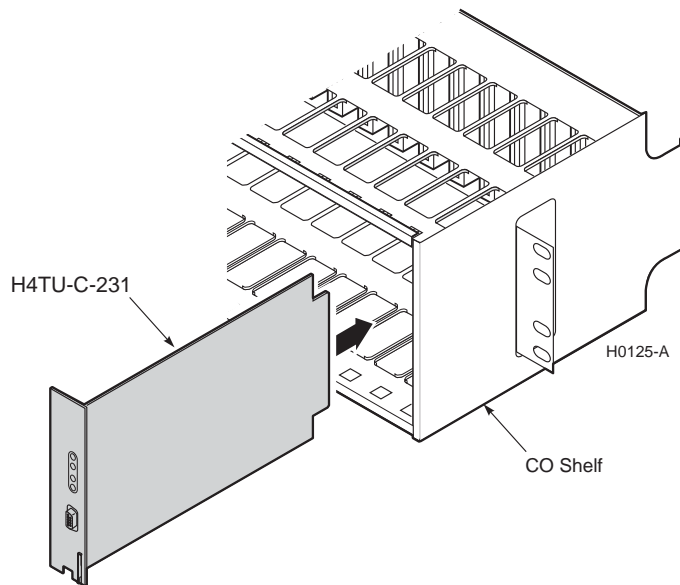
Figure 2. Installing an H4TU-C into a Shelf
