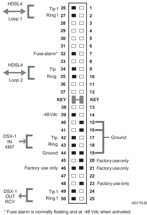
Figure 32. H4TU-C Card-Edge Connector
