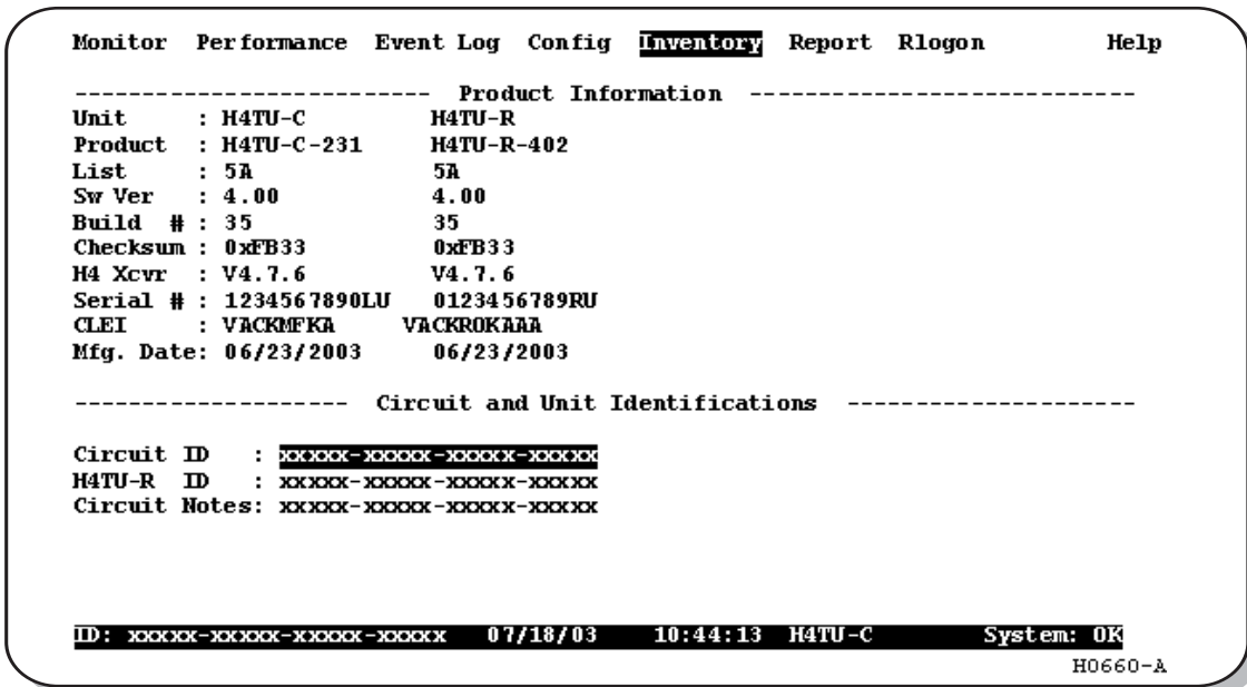
Figure 5. Inventory Screen
