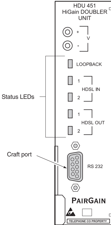
Figure 3. The HDU-451 List 4B Front Panel
