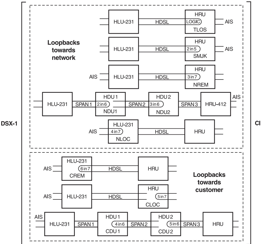
Figure 4. HiGain Loopbacks.
