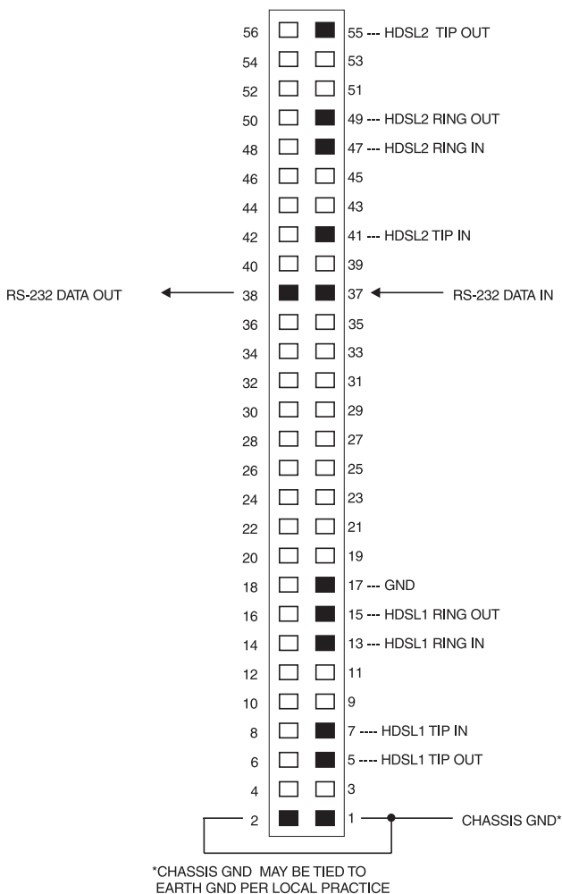
Figure 12. HDU-451 List 4B Pin-Outs (active pins are black).
