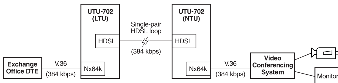
Figure 8. Single Pair Rate Selectable HDSL Video Conferencing Application
