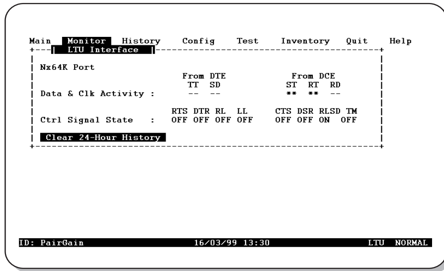
Figure 33. Monitor LTU Interface Screen
