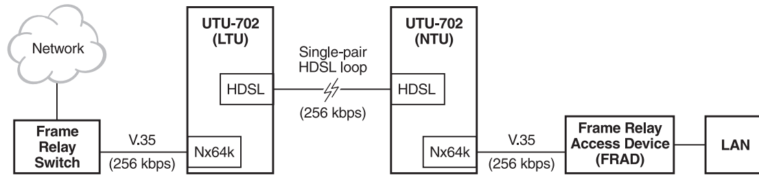
Figure 9. Single Pair Rate Selectable HDSL Frame Relay Application
