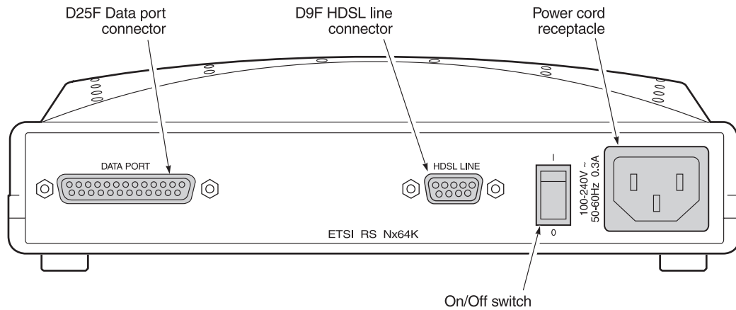
Figure 4. ETU-752C Desktop Unit Rear Panel
