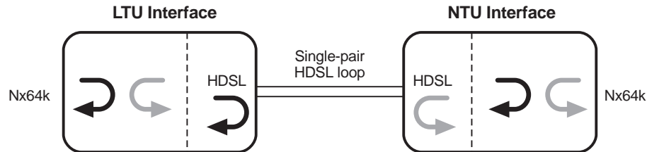
Figure 10. Loopback Operations
