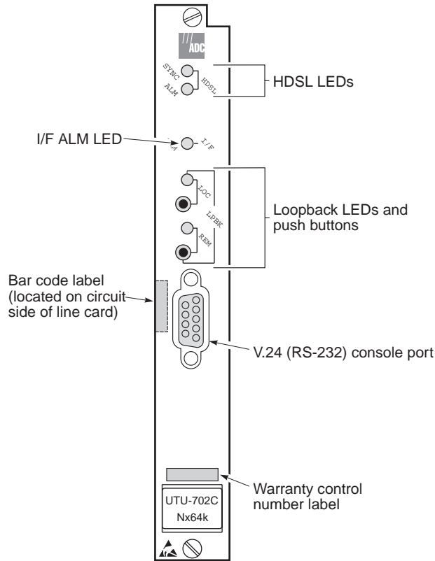
Figure 2. UTU-702C Line Unit Front Panel
