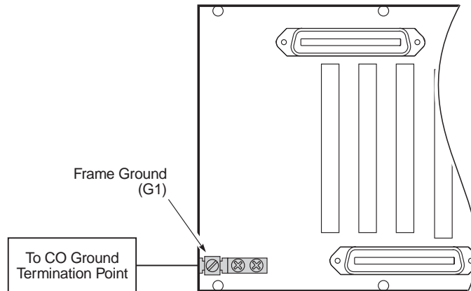
Figure 4. Connecting the Frame Ground (Protection Ground)
