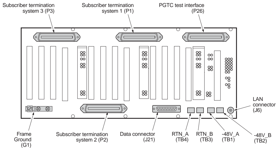
Figure 2. FCS-717 List 4B COT Shelf Backplane
