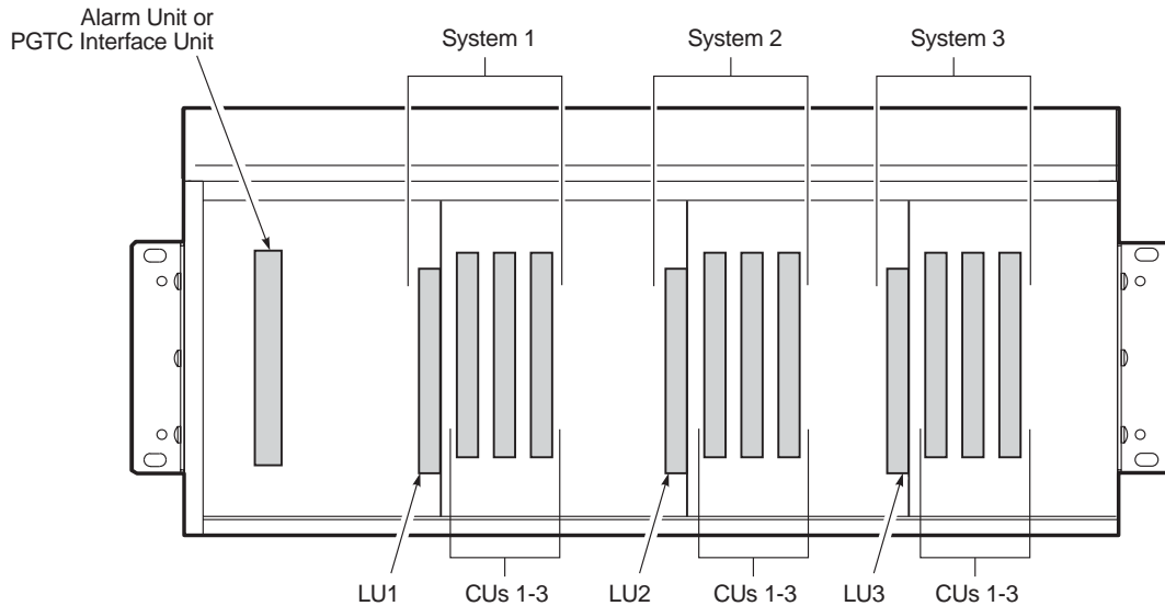
Figure 1. FCS-717 List 4B COT Shelf (Card-side, Front View)
