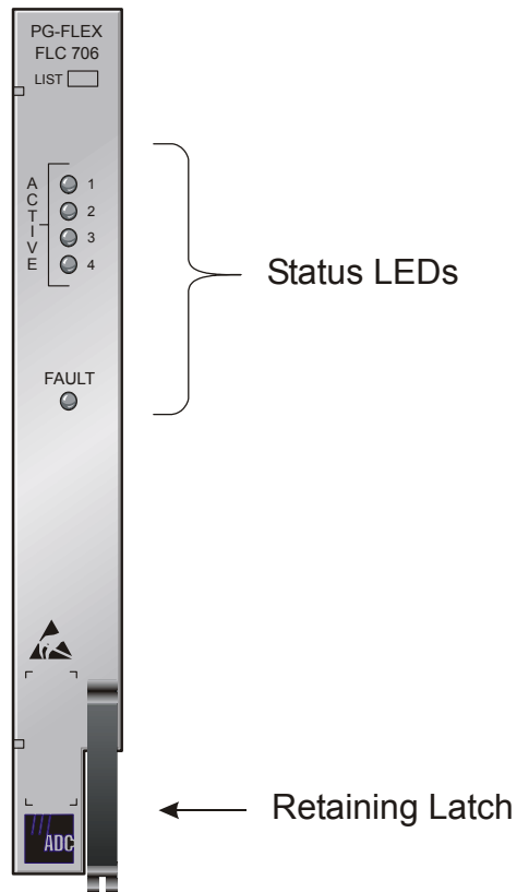
Figure 2. FLC-706 ISDN Channel Unit Front Panel
