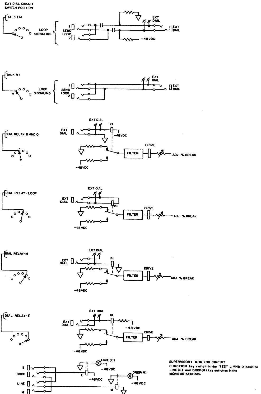
Figure 3-4 SUPERVISORY MONITOR CIRCUITS
